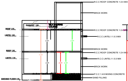
CROSS SECTION
