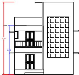
FRONT ELEVATION
