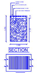
RAIN WATER HARVESTING PERCOLATION BED
