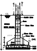
FOUNDATION DETAIL SCALE : 1:50.
