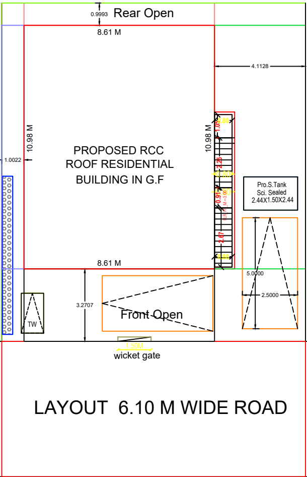
PLOT No.35 & 36
