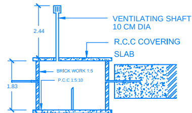
SEPTIC TANK DETAIL
