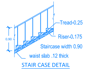
STAIR CASE DETAIL
