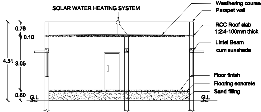
SECTION ON MK
