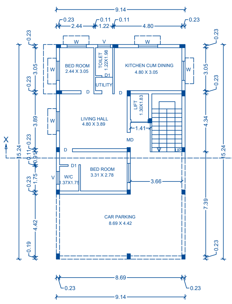
FLOOR PLAN
