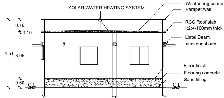
SECTION ON MK
