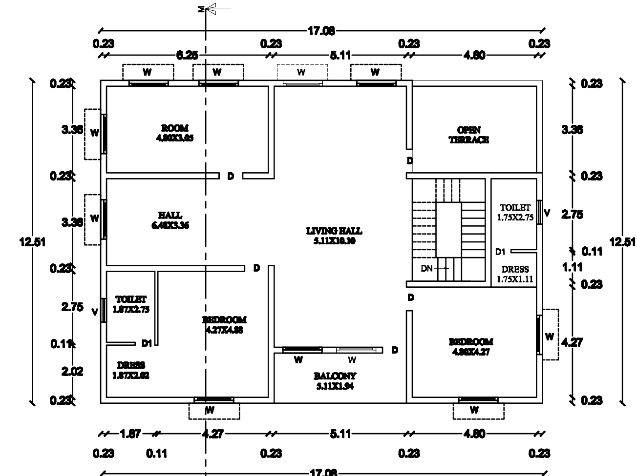
PRO- FIRST FLOOR PLAN
