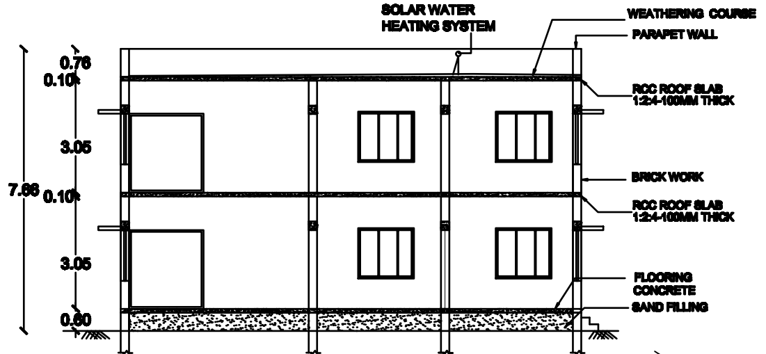
SECTION ON RM
