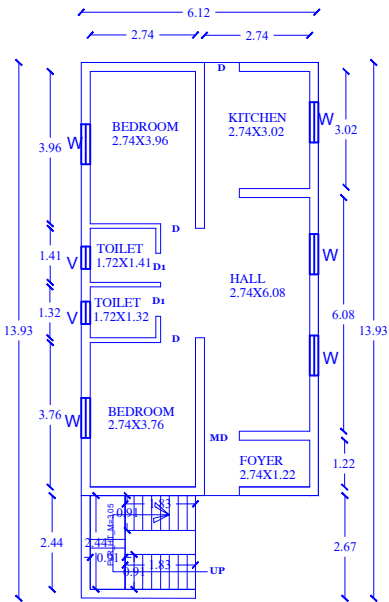
EXI-GROUND & PRO GROUND FLOOR PLAN
