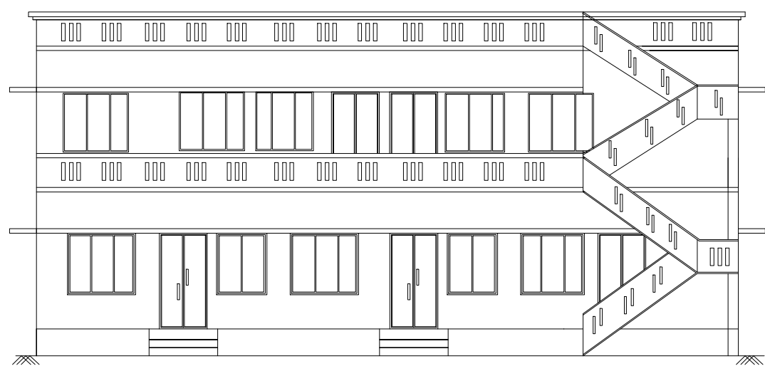
FRONT ELEVATION
