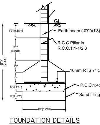
FOUNDATION DETAILS
