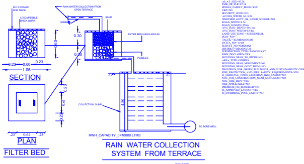
RAIN WATER COLLECTION SYSTEM FROM TERRACE
