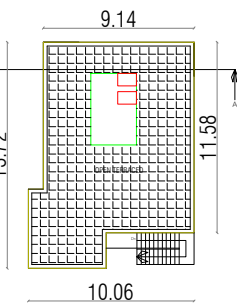
OPEN TERRACE PLAN
