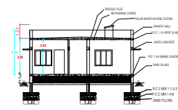
SECTION NO - "AA"
