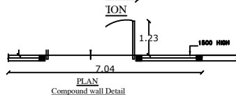
PLAN Compound wall Detail
