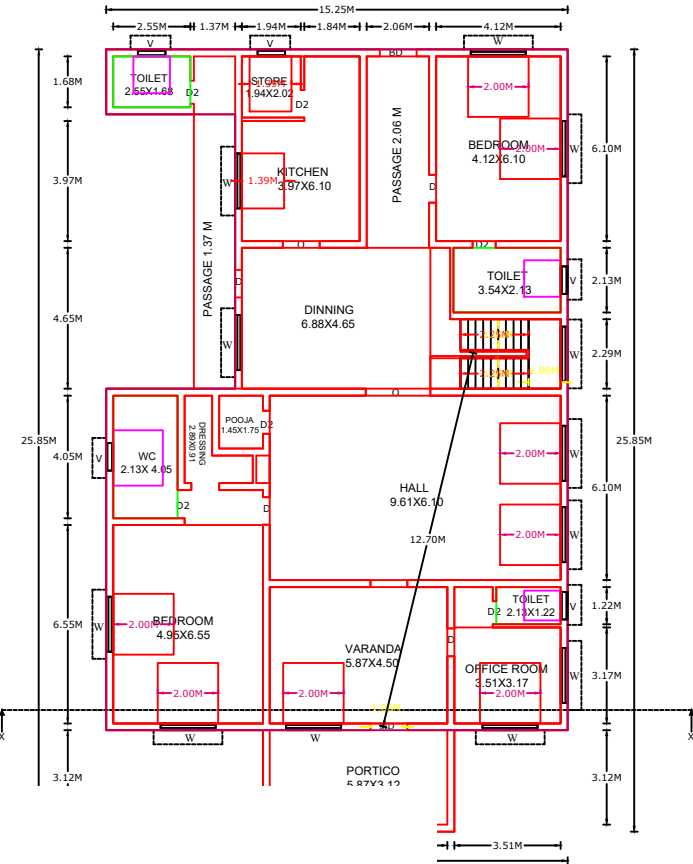
GR PLAN
