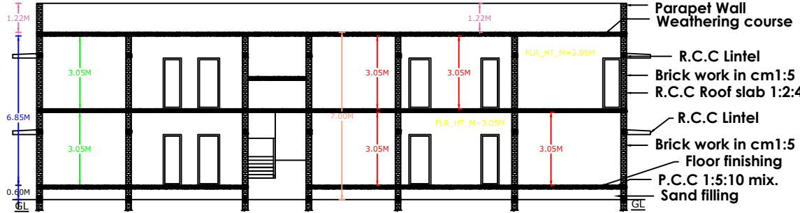
SECTION ON XX
