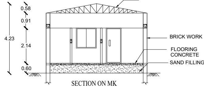
SECTION ON MK
