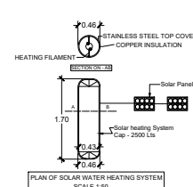
PLAN OF SOLAR WATER HEATING SYSTEM SCALE 1:50
