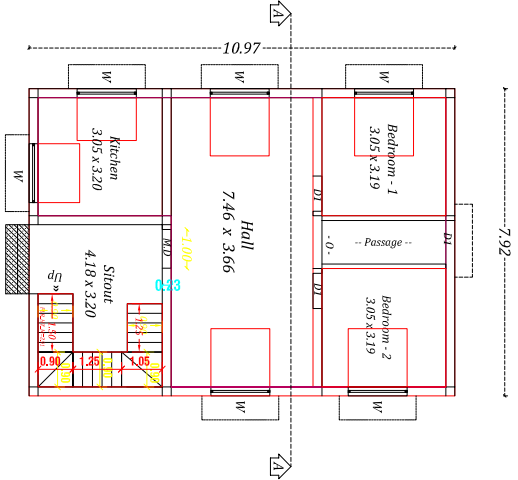
PRO. GROUND FLOOR PLAN
