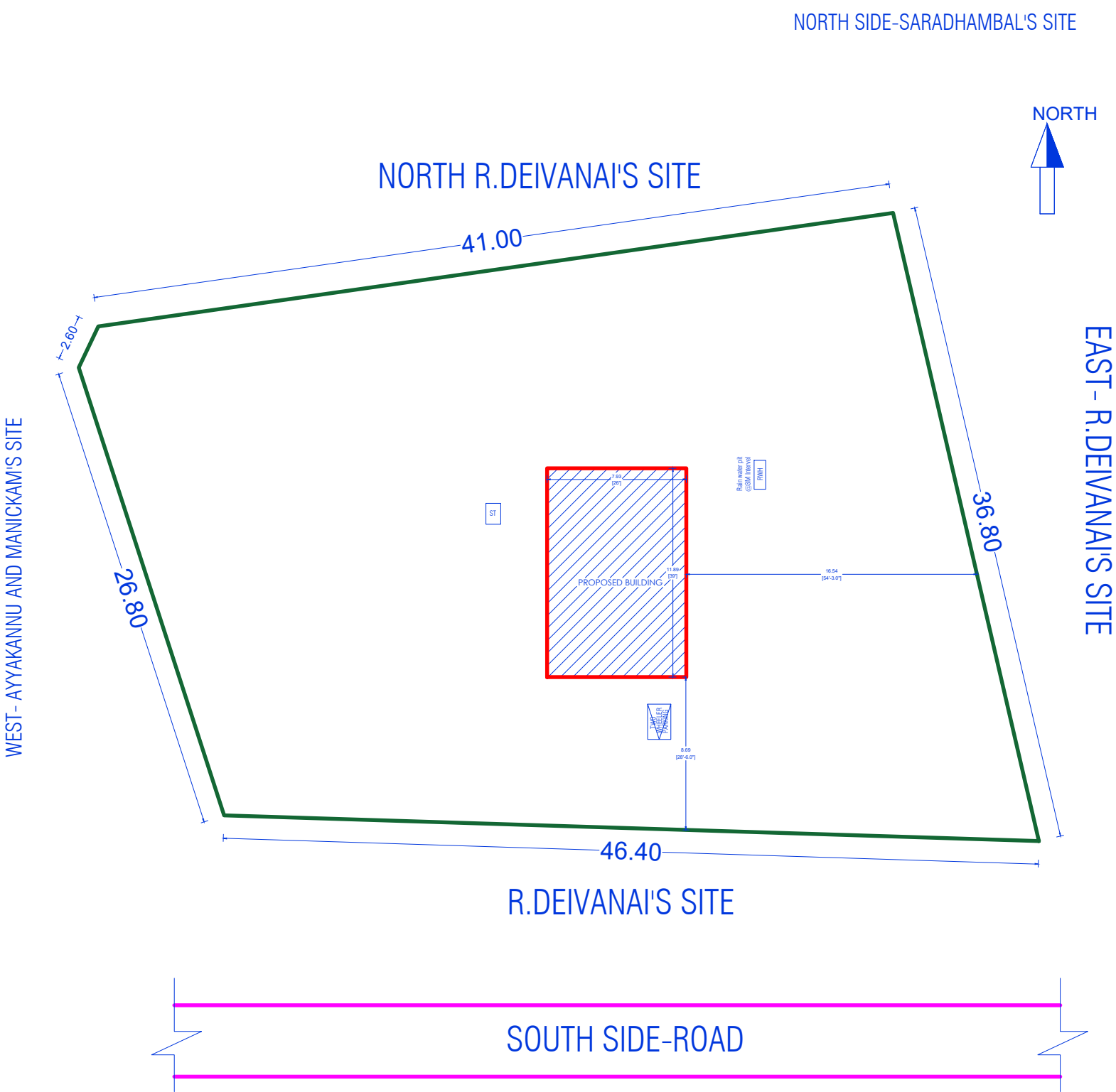
SITE PLAN
