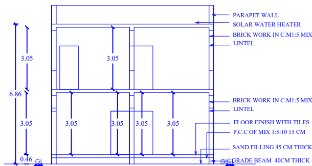
SECTION-AB
