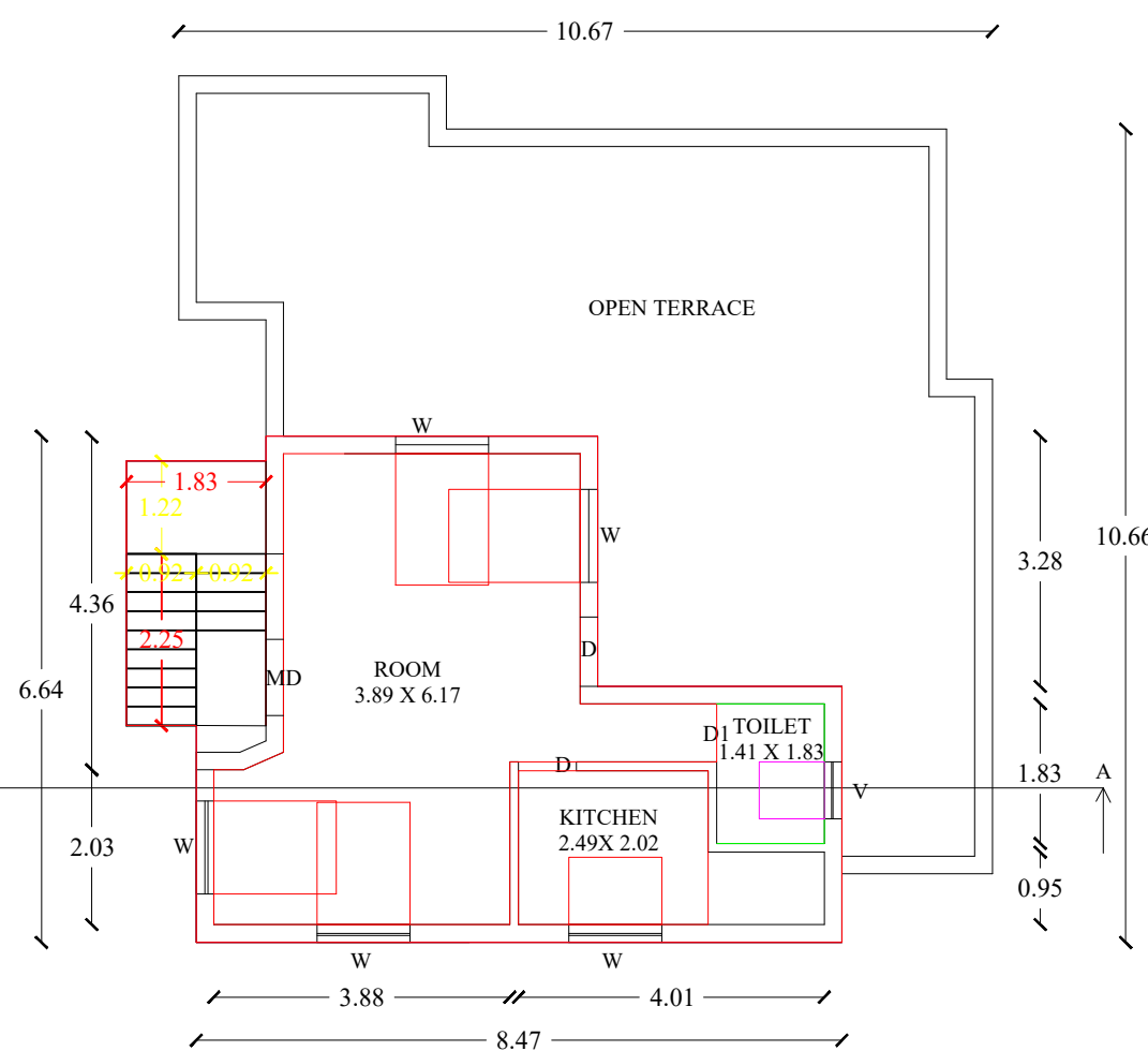
EXI. FIRST FLOOR PLAN
