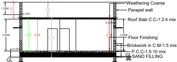
CROSS SECTION ON AB
