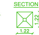
COLUMN DETAILS
