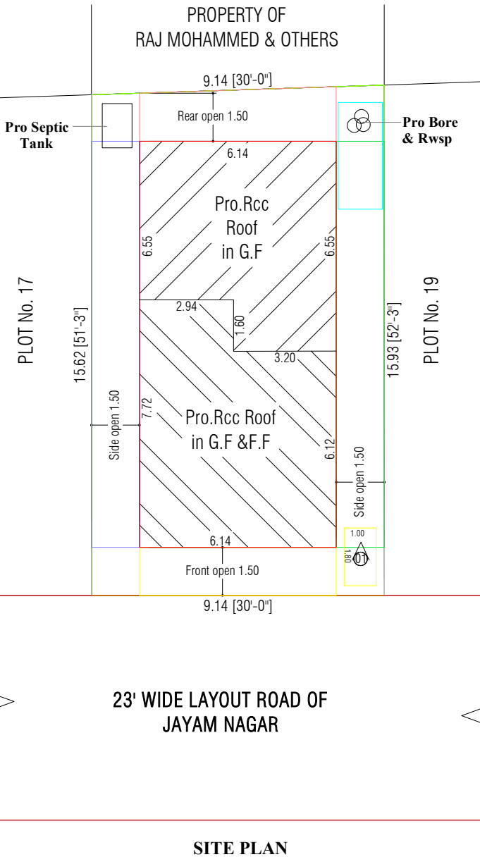
SITE PLAN
