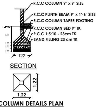
COLUMN DETAILS PLAN
