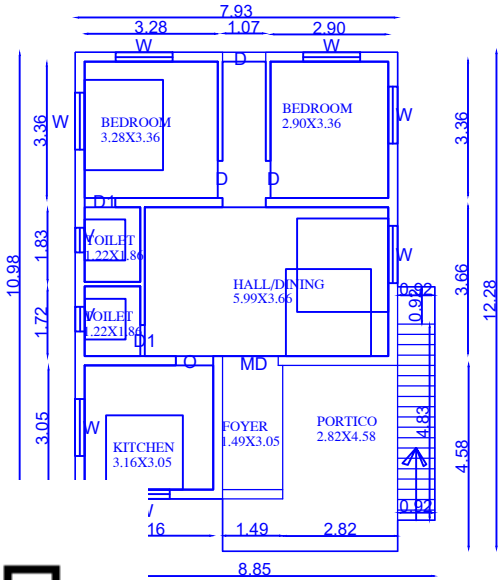
ND FLOOR PLAN
