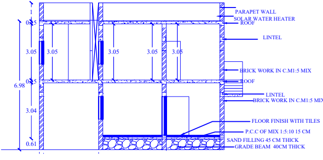
SECTION AA1
