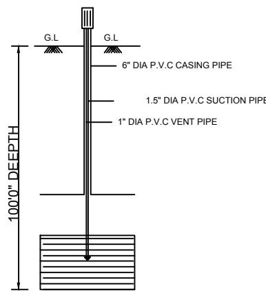
BORE WELL
