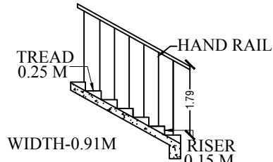
STAIRCASE DETAILS
