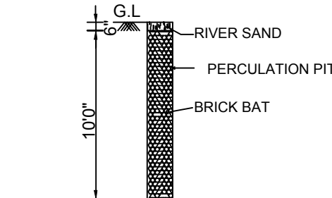
PERCOLATION PIT
