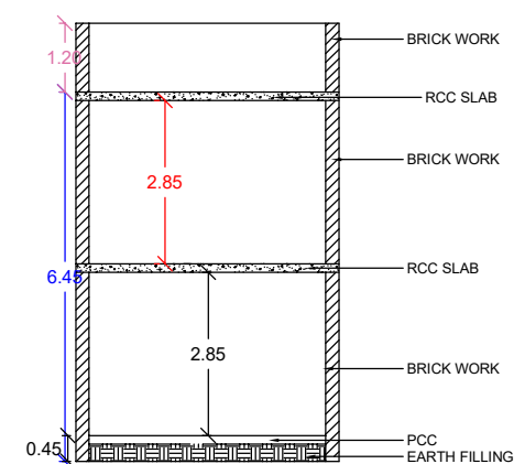
SECTION-XX
