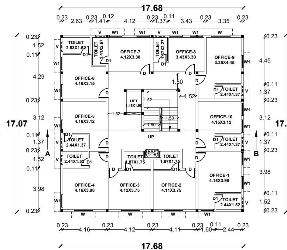
TYPICAL FLOOR PLAN FIRST,SECOND,THIRD FLOOR PLAN
