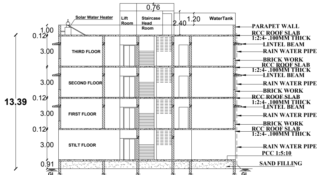
SECTION- AB
