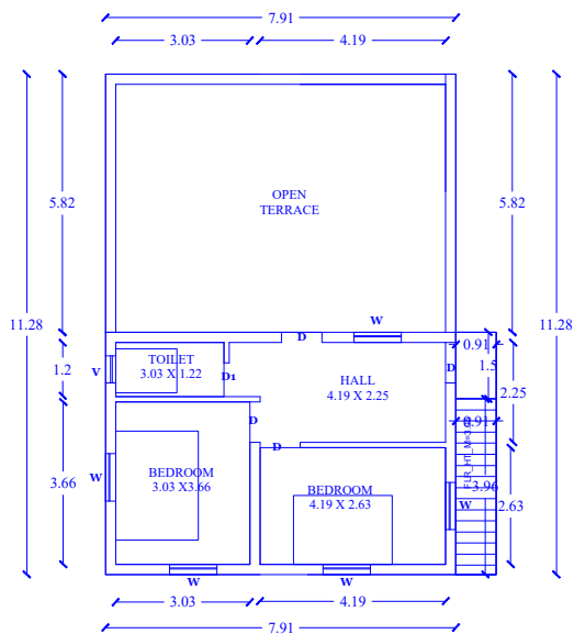
PRO. FIRST FLOOR PLAN
