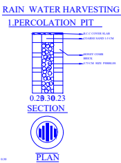
RAIN WATER HARVESTING PERCOLATION PIT
