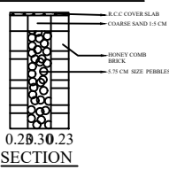
RAIN WATER HARVESTING 1.PERCOLATION PIT
