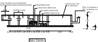
SECTION
