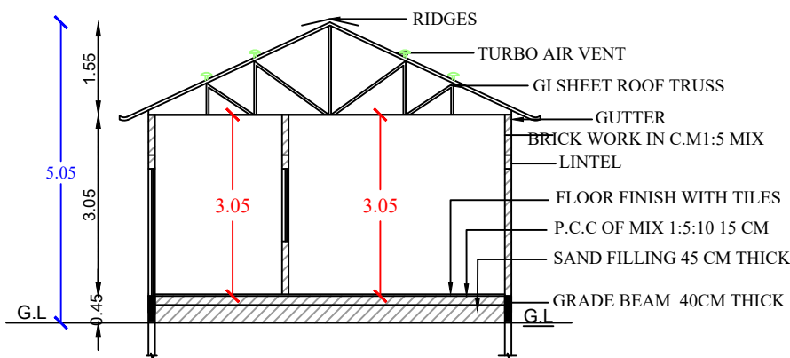
SECTION- AA1
