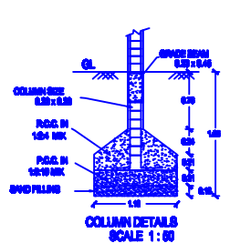
COLUMN DETAILS SCALE 1:50
