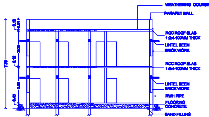
SECTION X-Y
