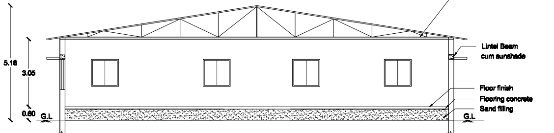
SECTION ON MK
