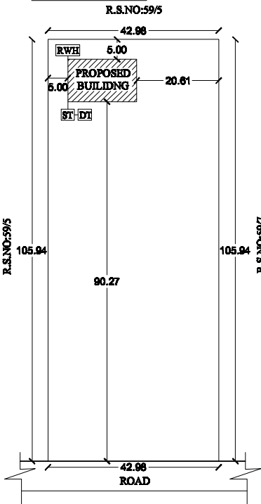
SITE PLAN SCALE 1:800
