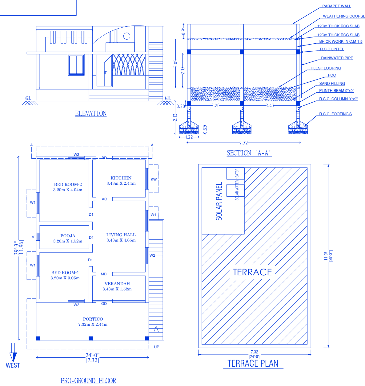
PRO-GROUND FLOOR
