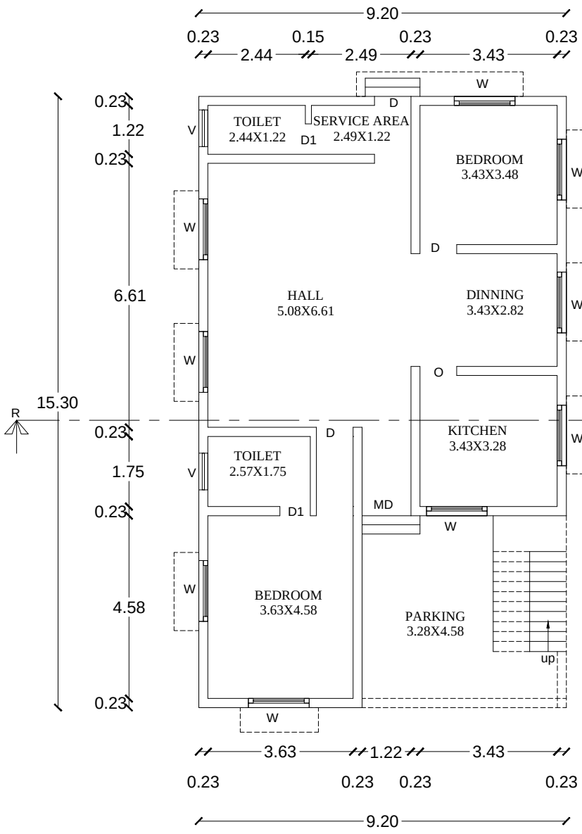
EXG- GROUND FLOOR PLAN
