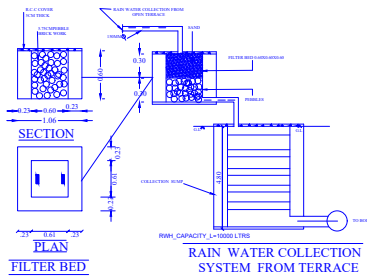
FILTER BED
