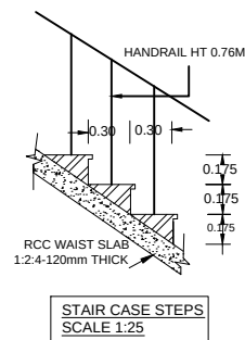
STAIR CASE STEPS SCALE 1:25
