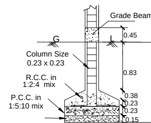
COLUMN DETAILS NOT TO SCALE
