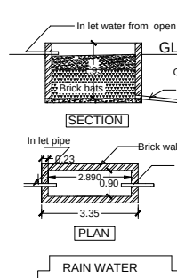
RAIN WATER HARVESTING TANK
