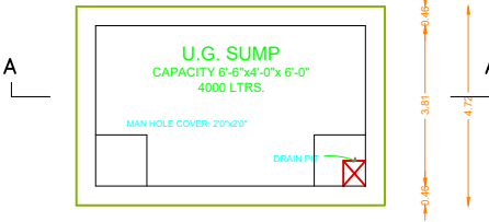
SUMP DETAIL
