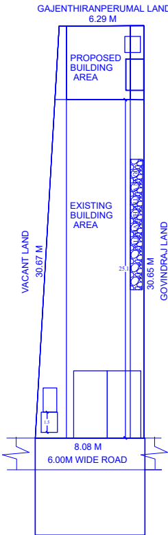
SITE PLAN SCALE 1:200
