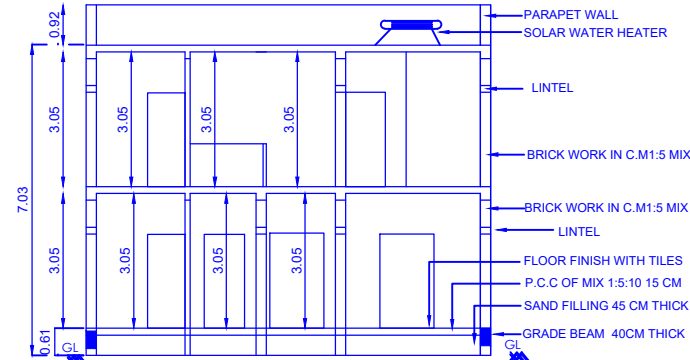
SECTION -A-A
