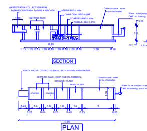
WASTE WATER RECYCLING SYSTEM
