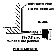
PERCOLATION PIT
