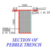
SECTION OF PEBBLE TRENCH
