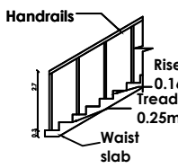
STAIRCASE DETAILS
