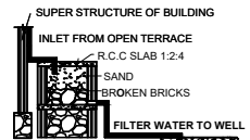
RAINWATER HARVESTING
