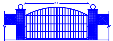
COMPOUND GATE (NOT TO SCALE)
