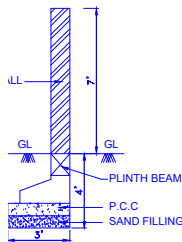
JND WALL DETAIL
