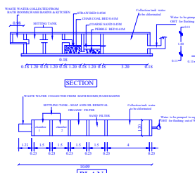
WASTE WATER RECYCLING SYSTEM
