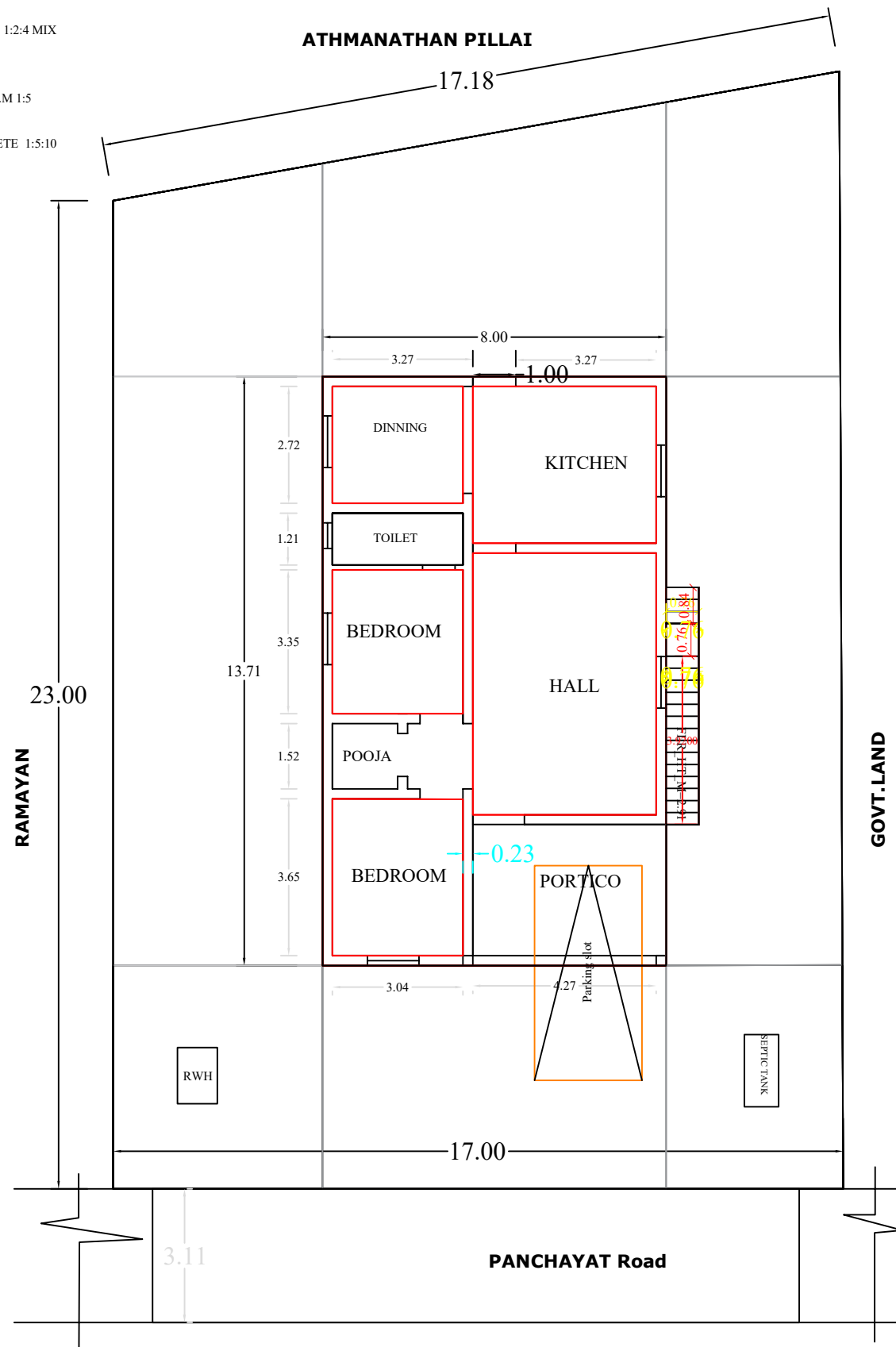
SITE PLAN AND GROUND FLOOR PLAN
