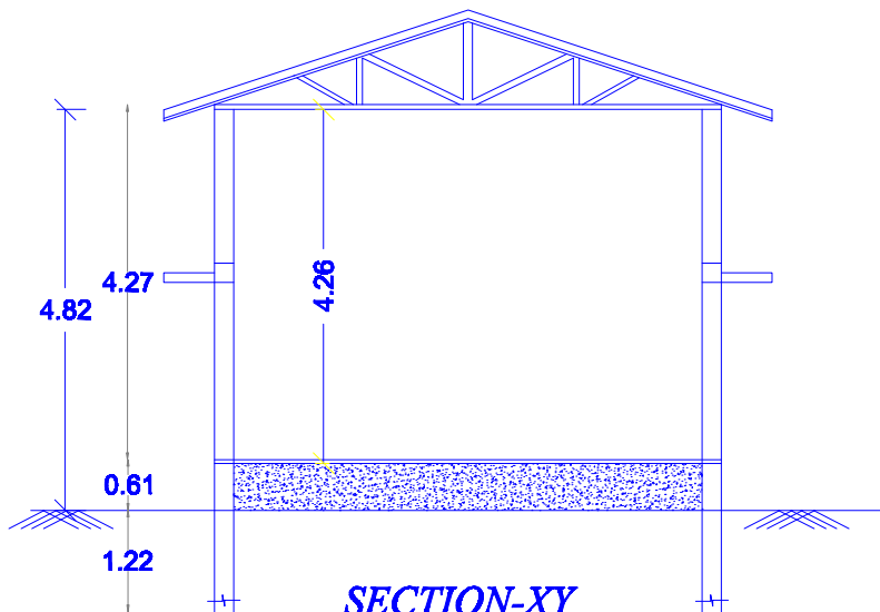
SECTION-XY
