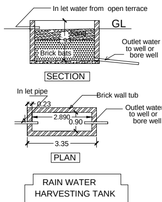
RAIN WATER HARVESTING TANK
