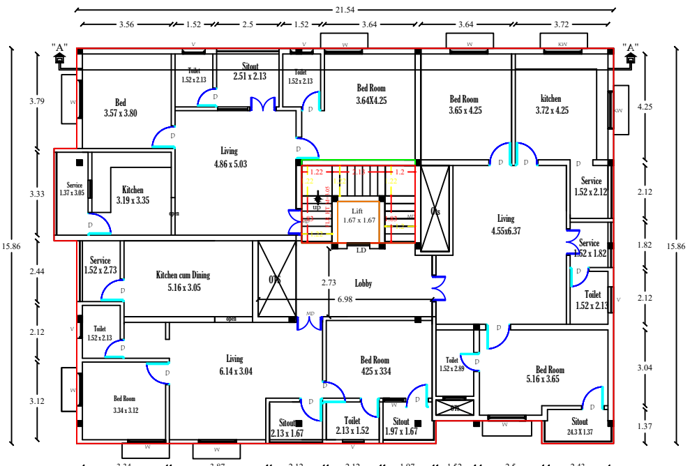
EXI - SECOND FLOOR PLAN
