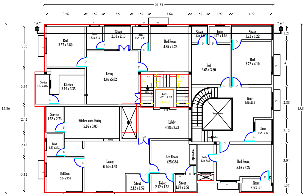
EXI - FIRST FLOOR PLAN
