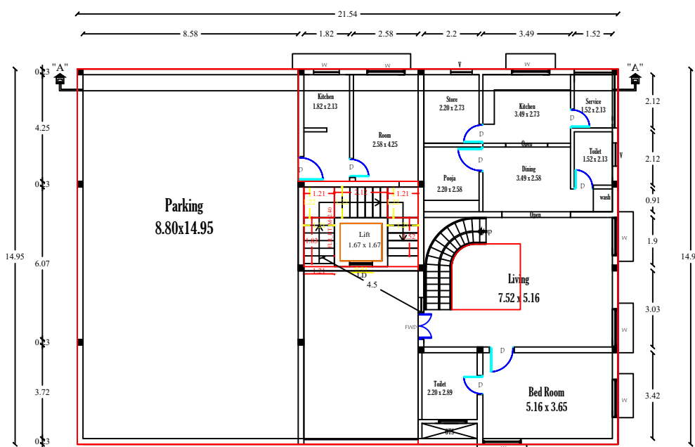
EXI-GROUND FLOOR PLAN
