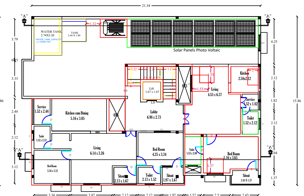
EXI - AND PRO -THIRD FLOOR PLAN
