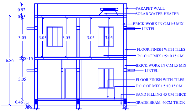
SECTION ON A-A1
