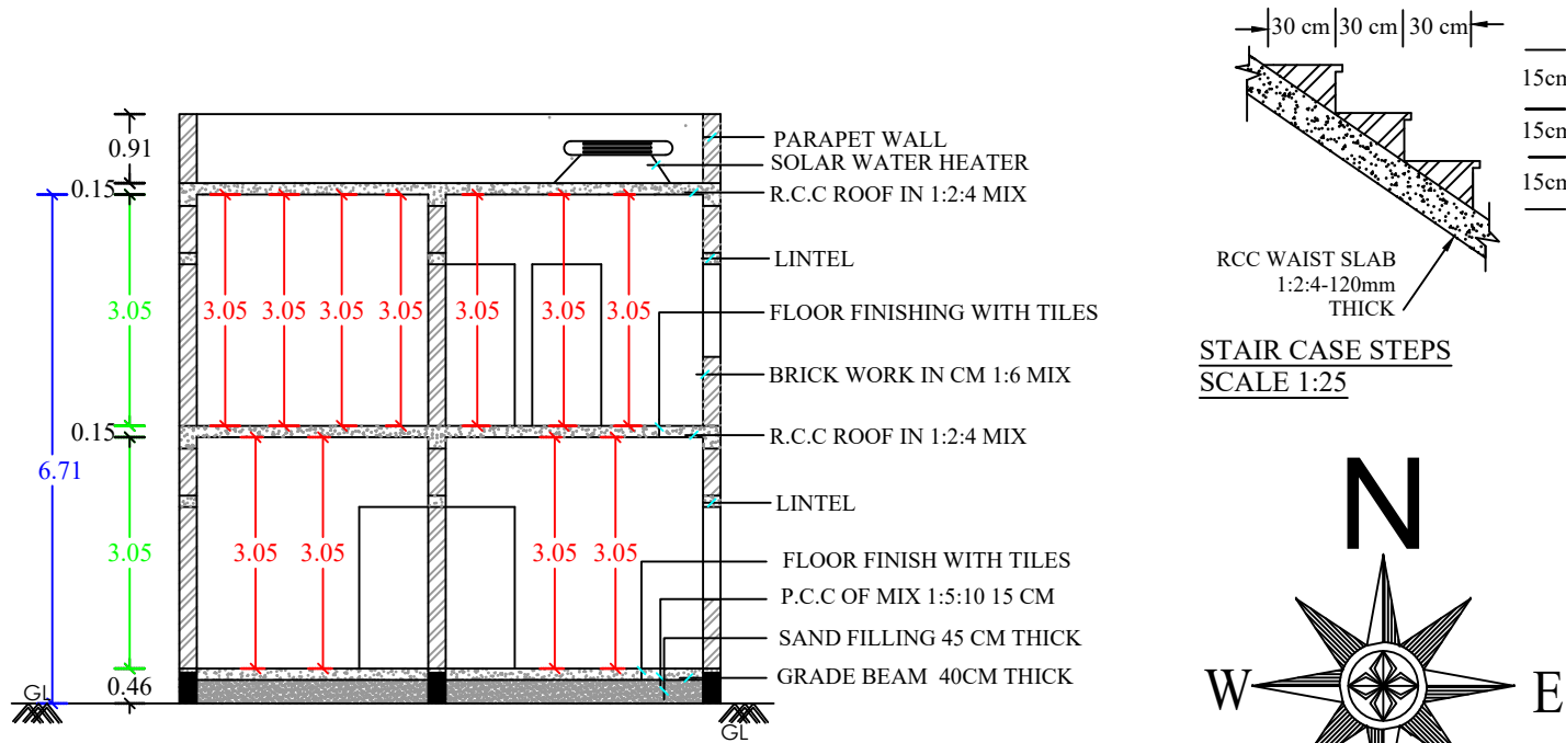
SECTION -AA'
