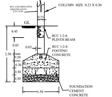
FOUNDATION DETAILS Scale 1:50
